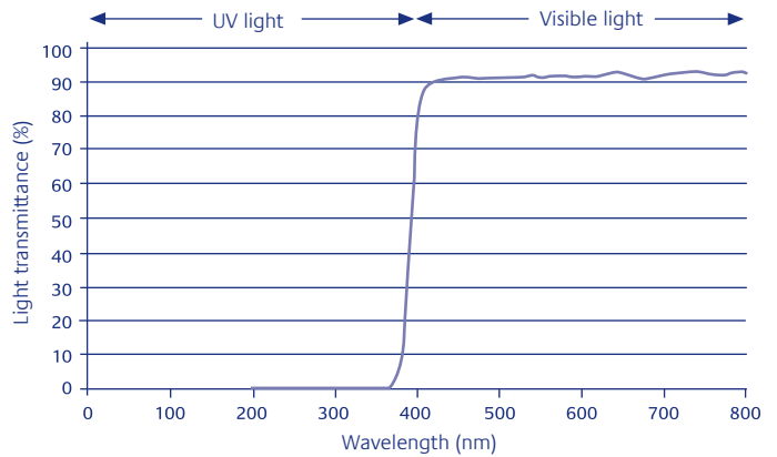
Figure 6 The unique proprietary technology applied to Lexan sheet blocks the UV rays of sunlight.
