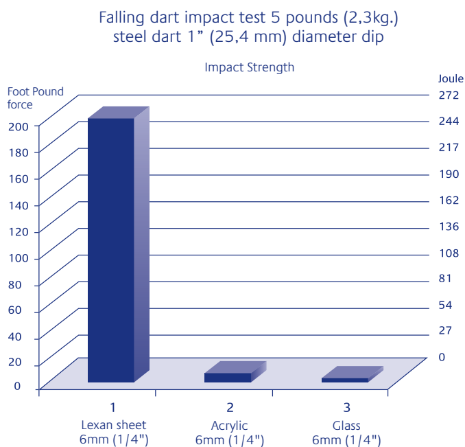
Figure 1 Impact resistance
